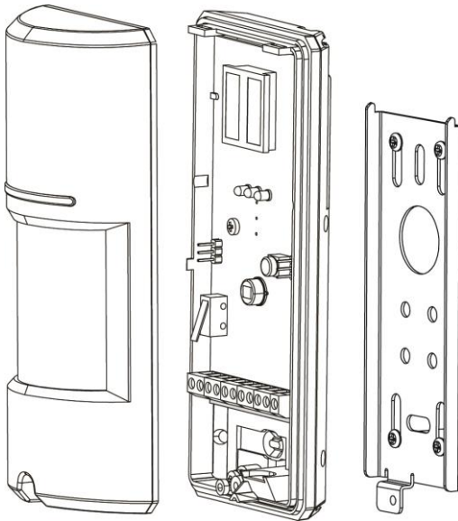
EDS-2000-AM Outdoor Motion Detector
